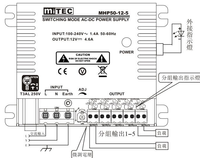
MHP50-12-5 接線示意圖:
