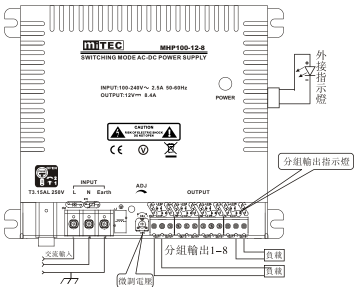
MHP100-12-8 接線示意圖:
